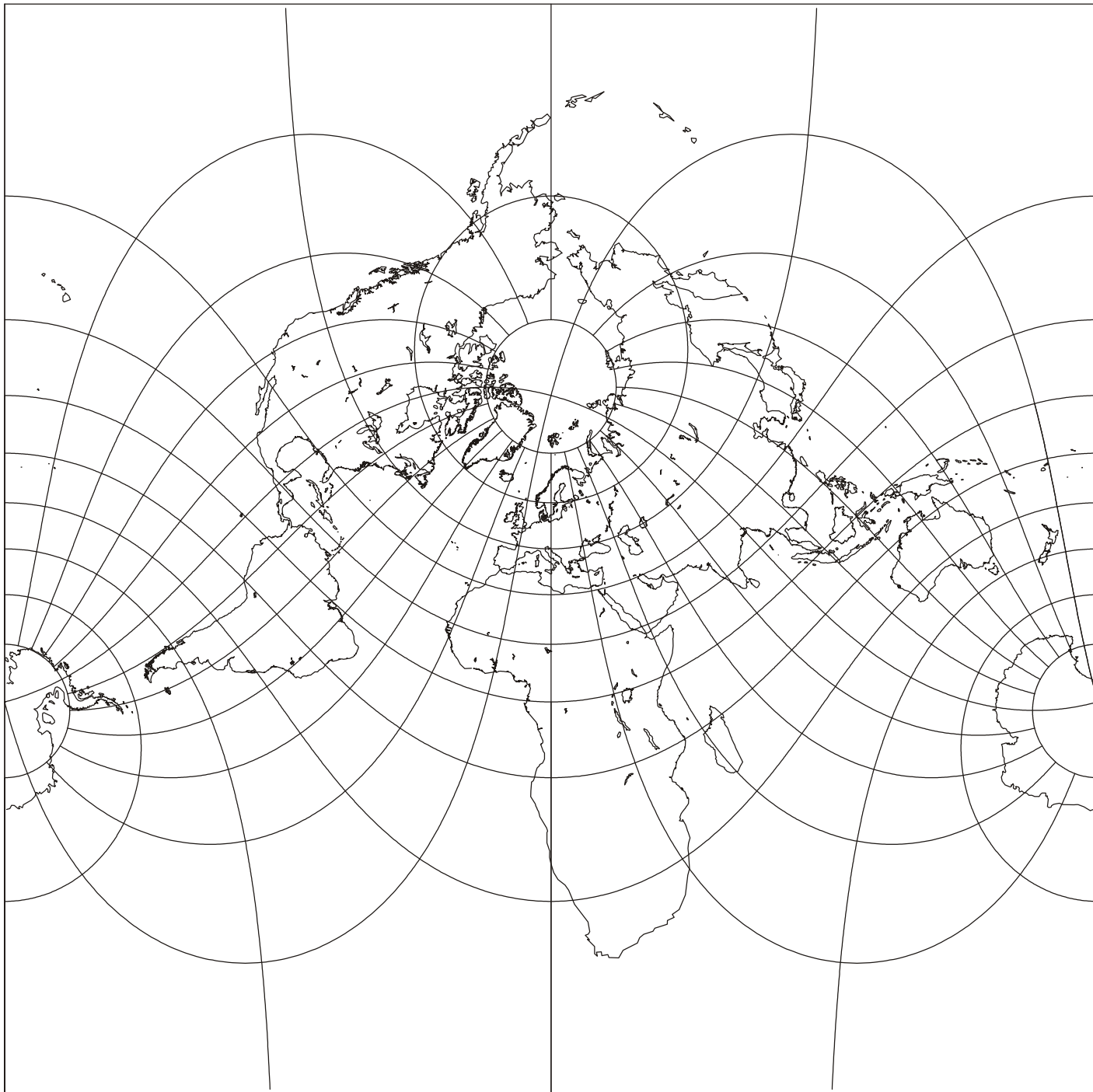
Oblique Mercator projection; Cylindrical; Conformal; C. S. Peirce; 1894
