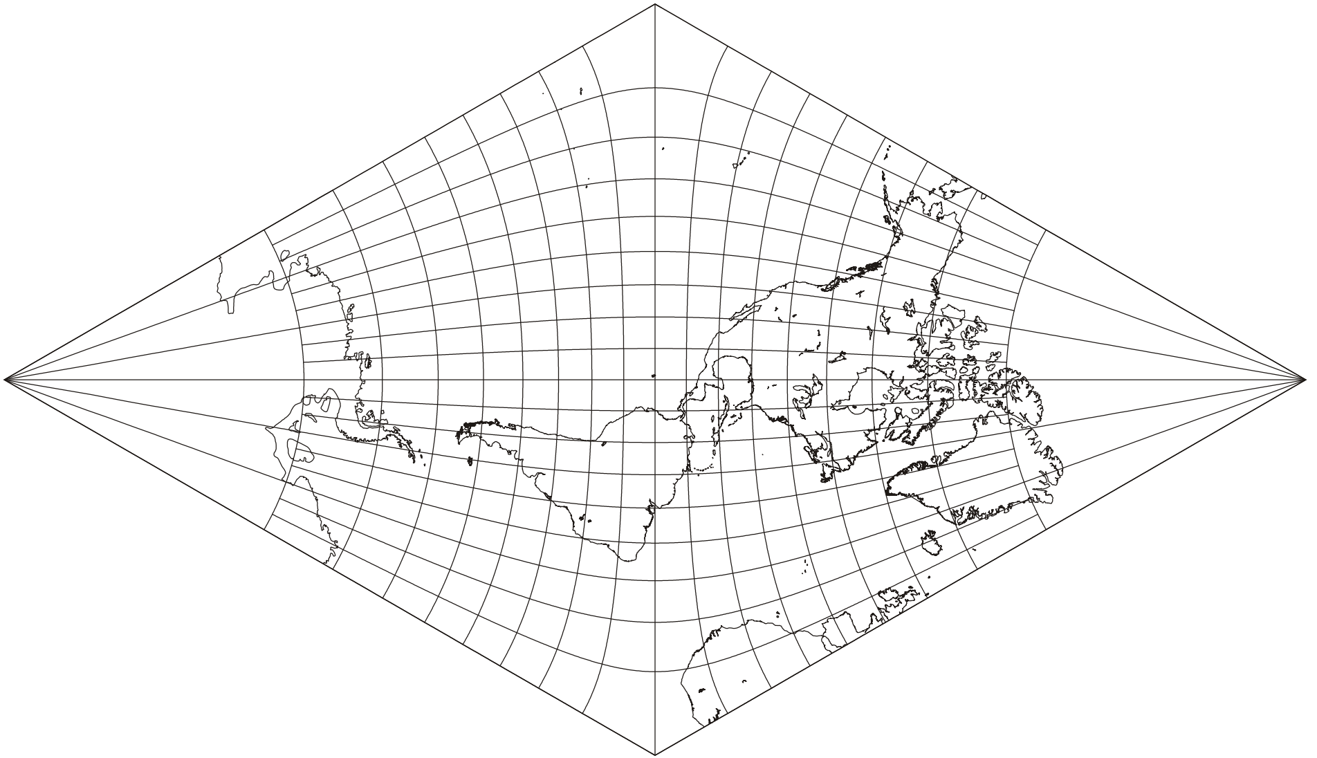
Rhombic projection; (Western Hemisphere, Poles in the 60 Deg. Angles); Miscellaneous; Conformal; Oscar S. Adams; 1925
