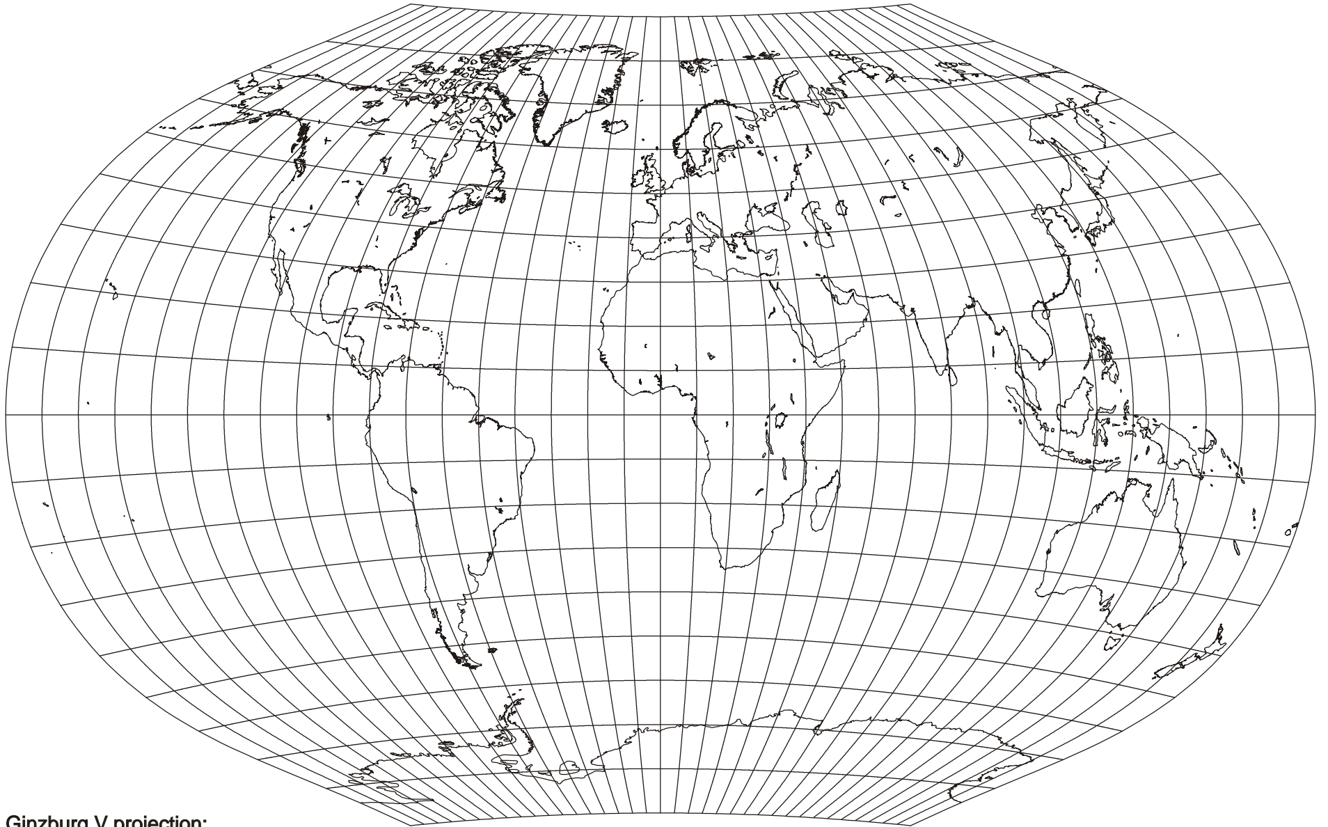
Ginzburg V projection; (TsNIIGAiK Modified Polyconic); Neither Conformal or Equal-area; G. A. Ginzburg; 1950
