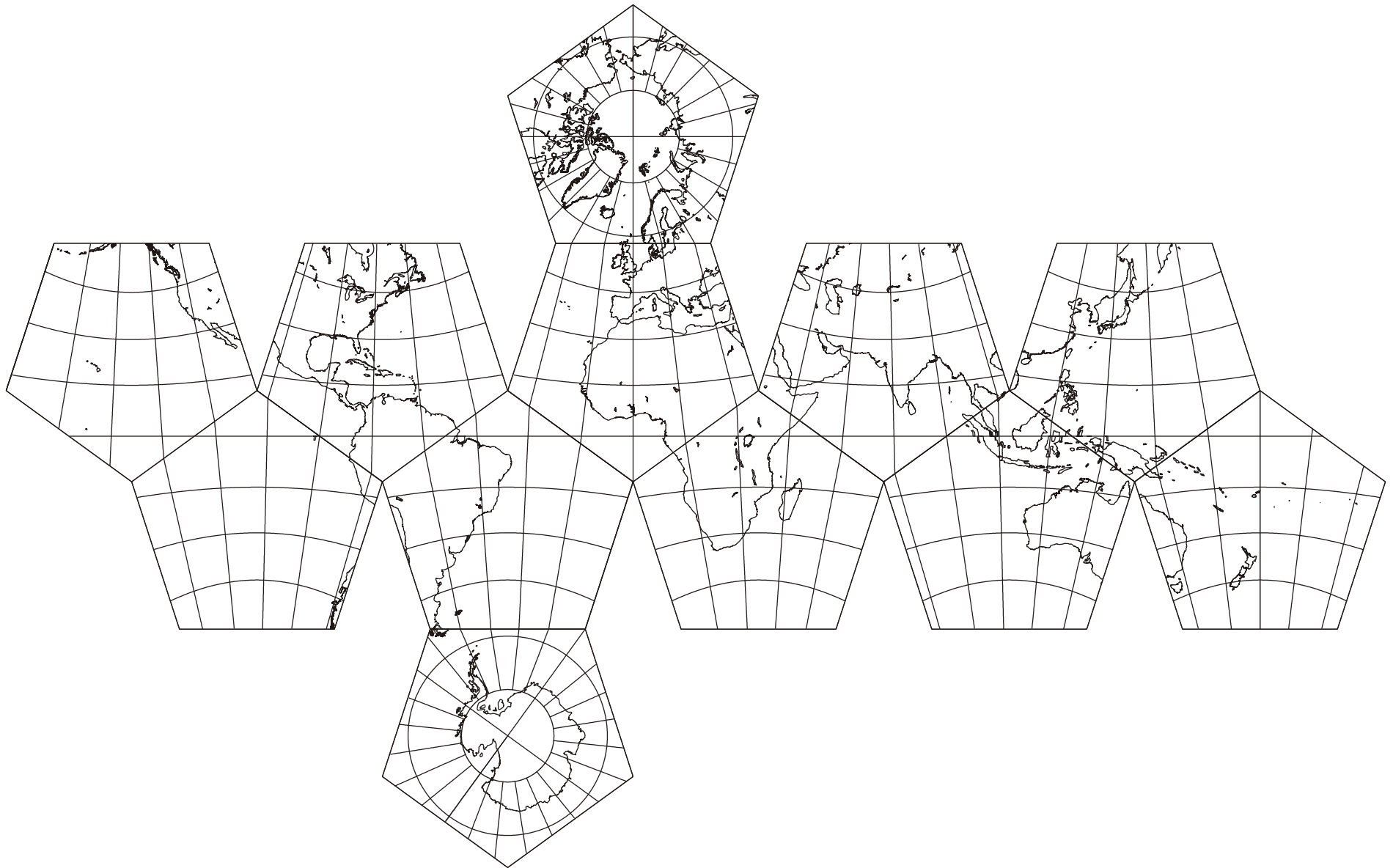
Gnomonic Dodecahedron; Polyhedral Globe; Platonic Solid; Source: John Parr Snyder's Personal Software
