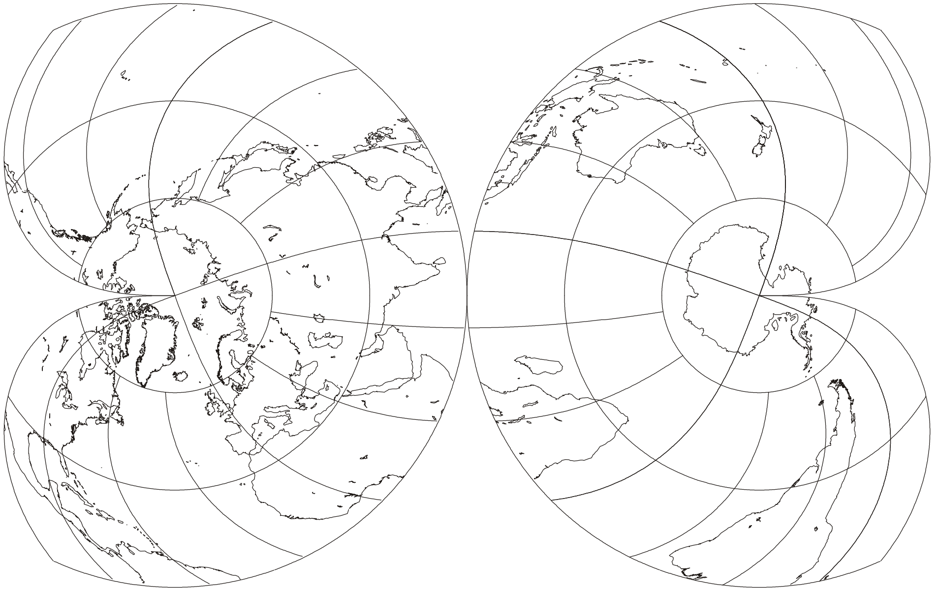
Double Cordiform projection; Pseudoconic; Equal-area; Oronce Finé; 1538
