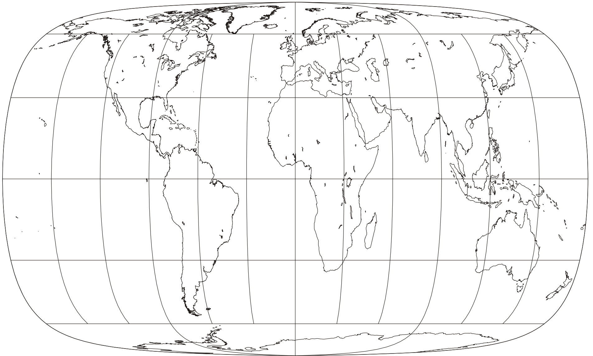
Baar projection; Pseudocylindrical; Equal-area; E. J. Baar, 1947
