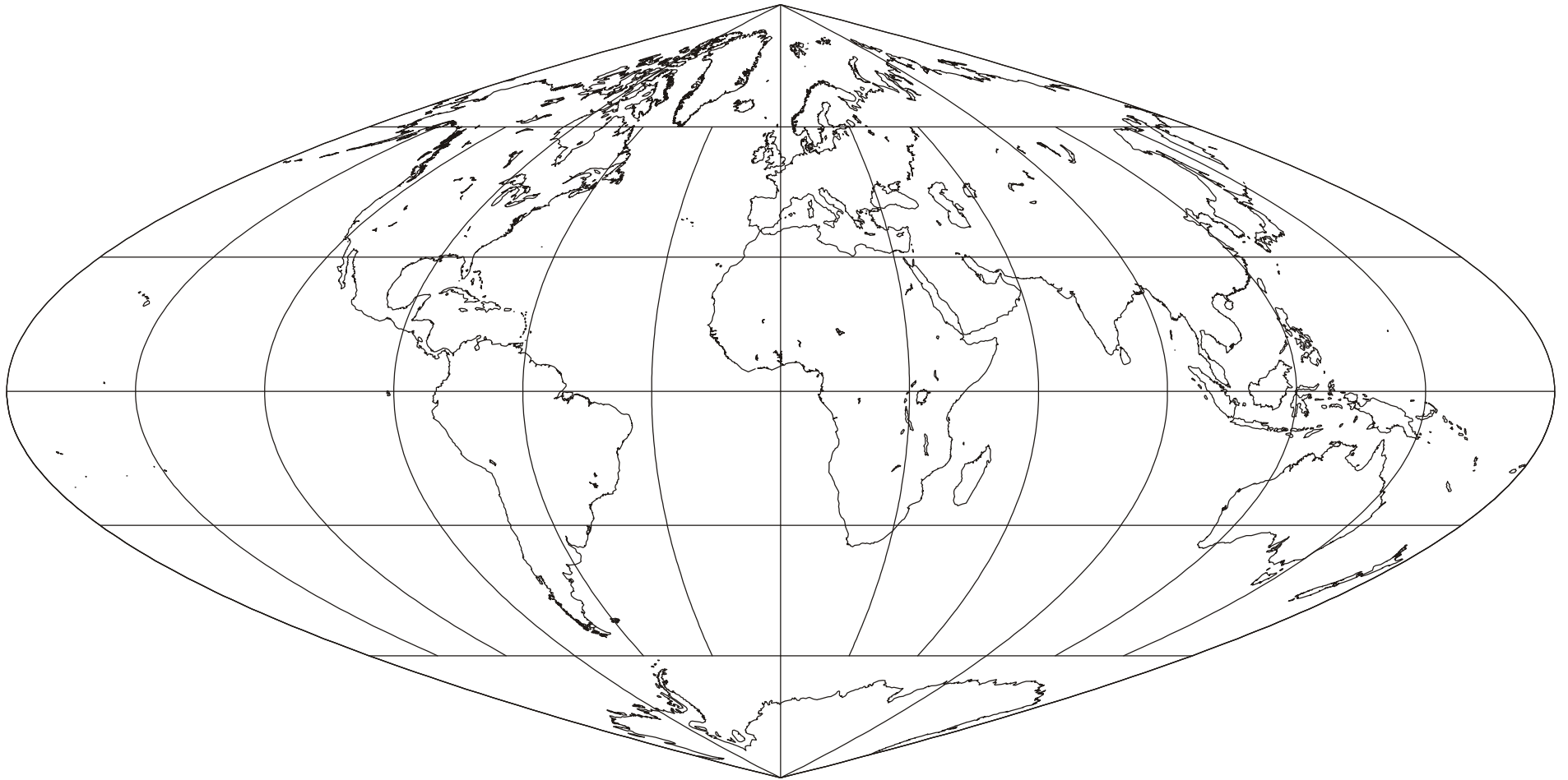
Craster Parabolic; Pseudocylindrical; Equal-area; J. E. E. Craster; 1929; Putnins (P4); 1934
